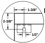
BRACKET DETAIL
