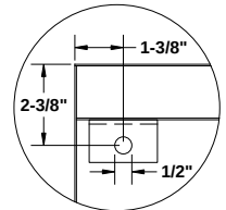
BRACKET DETAIL
