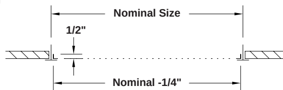
LAY ON PANEL ONLY STYLE D (Return)
