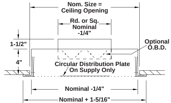
SURFACE MOUNT - STYLE B (Supply) Removable Face
