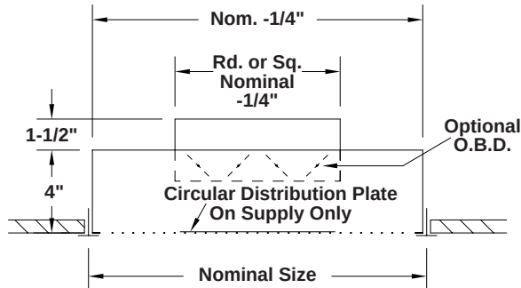
LAY ON T-BAR - STYLE A
