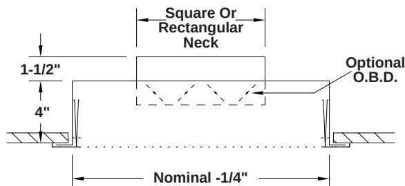
SURFACE MOUNT - STYLE B (Return) Removable Face
