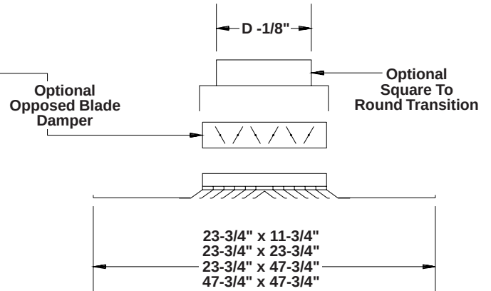
FRAME STYLE 2 – DIFFUSER IN LAY-ON T-BAR PANEL
