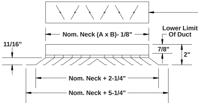
FRAME STYLE 1 – SURFACE MOUNTING
