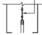
Option 6 2 Slot One-Way Blow Only - T-Extension Is Added To Fit Over Existing Grid T-Bar (By Others). Slot Provided In Ends
