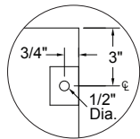
Hanger Bracket Detail
