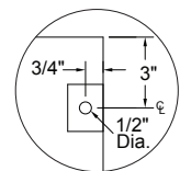
Hanger Bracket Detail
